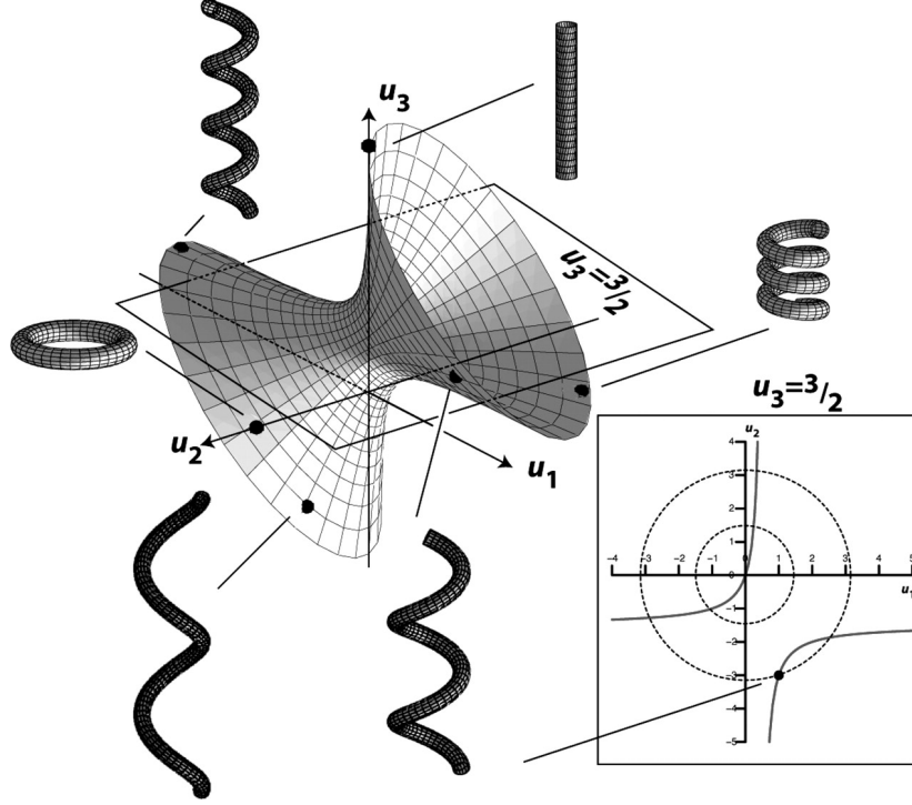
Figure 4: Homology, Helicity, and Hyperbolicity: a “geometric” Rosetta Stone. (Image Courtesy of Alain Goriely, “Helices” 2006)
