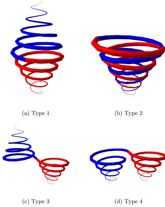
Figure 1: The THM_4 geometric family.
